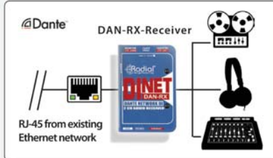
2-channels low-latency 24bit/96kHz audio over Ethernet
